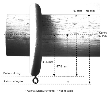
35 mm Pole and Ring
