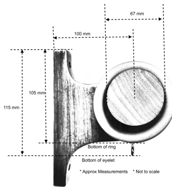
67 mm Architrave Bracket, pole and ring assembly
