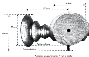
Tracked Top Fix Brackets 45mm
