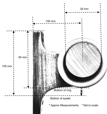
35 mm Architrave Bracket, pole and ring assembly
