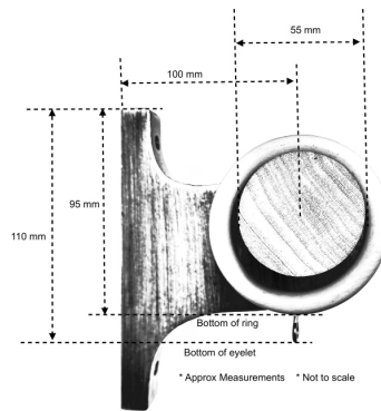
55 mm Architrave Bracket, pole and ring assembly
