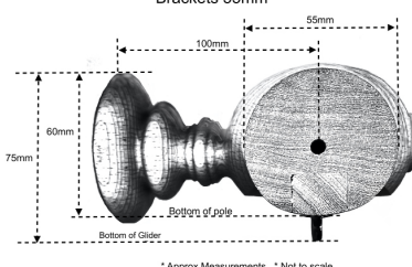
Tracked Top Fix Brackets 55mm
