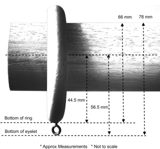
45 mm Pole and Ring
