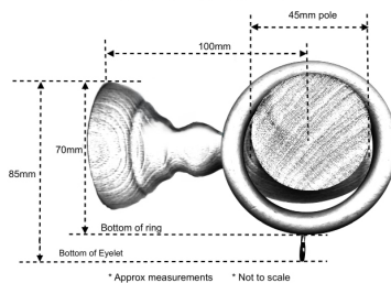
45 mm Cup Bracket, pole and ring assembly
