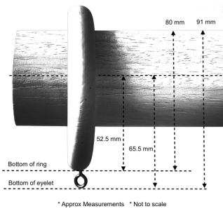
55 mm Pole and Ring
