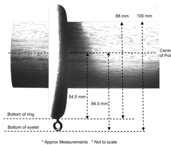
67 mm Pole and Ring
